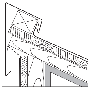
Detail First: Pultdach
